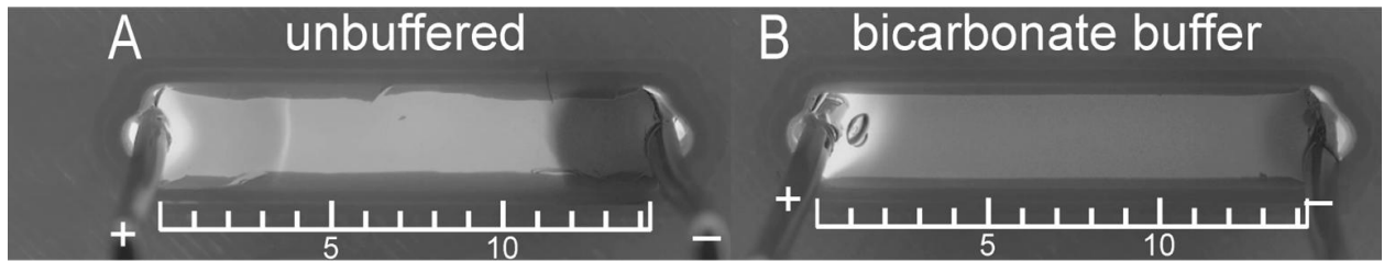
Figure 3: Changes in agarose gel pH following 8 rectangular pulses (10 ms duration, 400 V amplitude, 1 \text{ s}^{-1} repetition rate), performed in (A) unbuffered medium and (B) bicarbonate buffer medium. In order to observe also the effects of the diffusion, gels were photographed 60 seconds from the start of the delivery of the first pulse. Note that the scale bar dimensions are expressed in mm. Adapted from [6].
